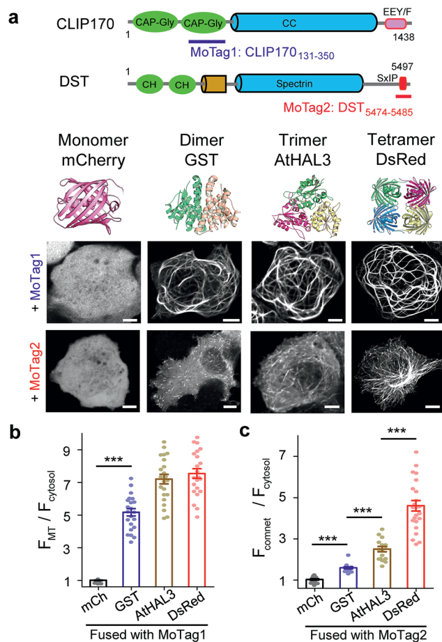
Fig. 1 MoTags can be used to discriminate well-known oligomeric proteins. (a) Representative confocal images of mCherry (mCh) or the indicated oligomeric proteins (GST as dimer, AtHAL3 as trimer and DsRed as tetramer) fused to either MoTag1 or MoTag2. The domain architectures of MoTag1 and MoTag2 are shown on the top. See Fig. S1† for the design and screening procedures. Scale bar, 5 \mu m. (b and c) Quantification of the MT-to-cytosol ( F_{MT}/F_{cytosol} ; b) or comet-to-cytosol fluorescence intensity ratio ( F_{comet}/F_{cytosol} ; c) in HeLa cells expressing monomeric or oligomeric MoTag1 (b) or MoTag2 (c). See Fig. S4–9† for more images and statistical analyses. n = 18 cells from three independent experiments. All data are shown as mean \pm s.e.m. *** P < 0.001 (two-tailed Student's t -test).
