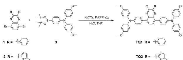
Scheme 1 The straightforward synthetic routes to TQ1 and TQ2 .
