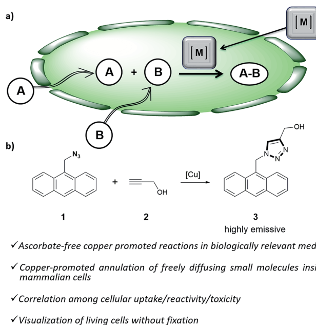
Fig. 1 (a) Outline of a metal-promoted bimolecular coupling of exogenous molecules in living cells; (b) CuAAC reaction between anthracenyl azide 1 and propargyl alcohol 2.
