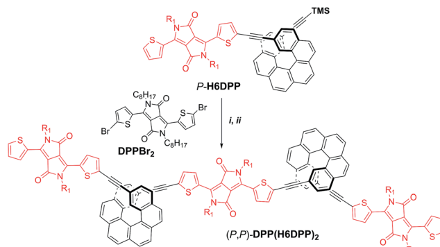
Scheme 2 Synthesis of enantiopure ( P,P )- DPP(H6DPP) 2 . TMS = trimethylsilyl. Reaction conditions: (i) TBAF, CH 2 Cl 2 , rt; (ii) Pd(PPh 3 ) 4 , CuI, Et 3 N/toluene, 50 °C, DPPBr 2 , 65%.
