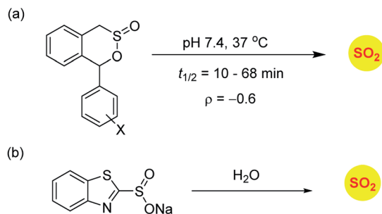
Scheme 10 Sulfonate based SO 2 donors.
