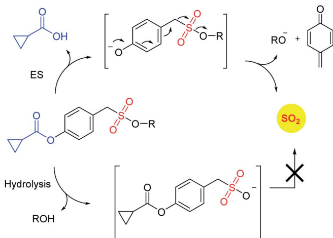
Scheme 11 Esterase activated SO 2 donors.
