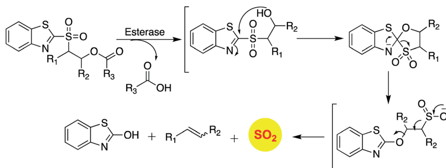
Scheme 12 Esterase activated SO 2 donors based on Julia olefination.
