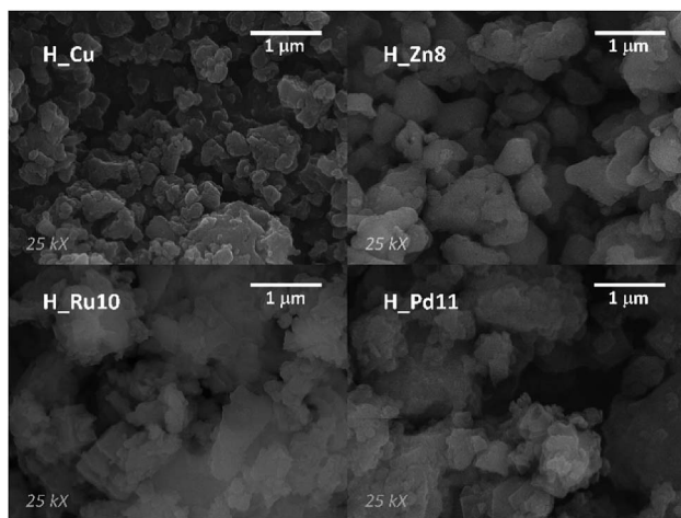
Fig. 2 SEM micrographs (SEI mode) at 25 000 magnifications of H_Cu, H_Zn8, H_Ru10, and H_Pd11.
