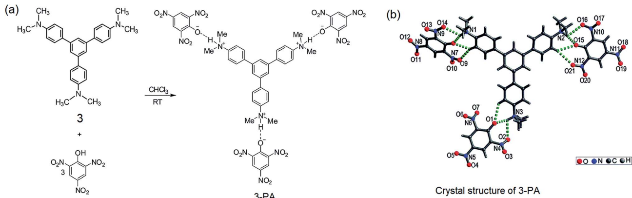
Scheme 2 (a) Preparation of the 3 –PA complex in a 1 : 3 stoichiometry. (b) Crystal structure of 3 –PA; hydrogen bonds are indicated by green dotted bonds. Reproduced from ref. 8 with permission. Copyright© 2015, Royal Society of Chemistry and the Centre National de la Recherche Scientifique.
