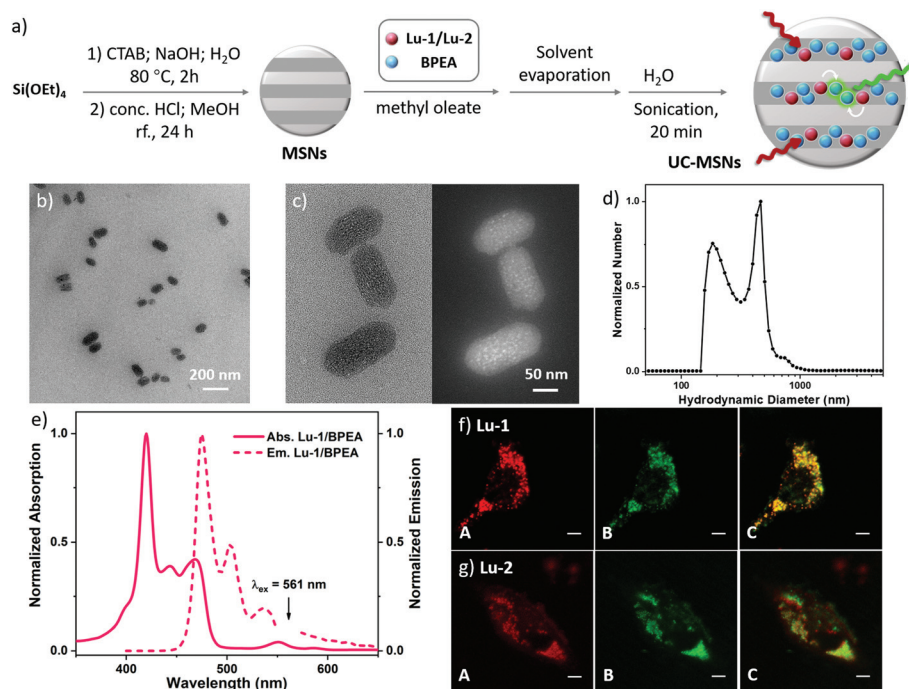
Fig. 5 (a) Illustration of the preparation scheme of UC-MSNs, and the sketch of the TTA-UC process in a single UC-MSN. (b) Transmission electron microscopy (TEM) image at 25 \times magnification, (c) bright field (left) and dark field (right) TEM image at 60 \times magnification, and (d) dynamic light scattering (DLS) of Lu-1/BPEA loaded UC-MSN. (e) Normalized absorption and emission spectra of Lu-1/BPEA loaded UC-MSN in water under an ambient atmosphere ( \lambda_{\text{ex}} = 561 \text{ nm} , 480 \text{ mW cm}^{-2} ). (f and g) Confocal fluorescence images of living HeLa cells with UC nanoparticles by a 455–525 nm channel under laser excitation at (A) 405 nm (red, prompt fluorescence); (B) 543 nm (green, upconverted fluorescence); and (C) merged images of (A) and (B). Rows f and g: images of UC-MSNs (incubated for 15 min) loaded with (f) Lu-1/BPEA and (g) Lu-2/BPEA (Presented with fake color; scale bar presents 20 \mu\text{m} ).
