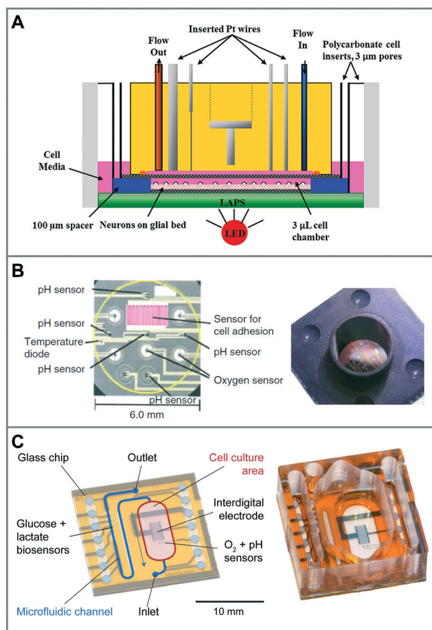
Fig. 5 Sensor systems for metabolic monitoring in 2D dynamic culture (microphysiometers). Cells are cultured directly on microsensors chips. For measurement, the medium volume is reduced to a few microliters and periodically exchanged by microfluidics. A: The Cytosensor microphysiometer based on a silicon chip, in which pH is measured with a light-addressable potentiometric sensor (LAPS). Amperometric microsensors are included by integrating wires in the cover. 111 (reprinted with permission, Copyright 2012 American Chemical Society). B: Silicon-based system with planar sensor integration for pH (ISFET), oxygen (amperometric) and cellular adhesion (interdigital electrode) 56,115 (reprinted with permission from Elsevier). C: Glass-based system for better microscopy with in situ amperometric oxygen sensors (platinum), potentiometric pH sensors (iridium oxide) and an interdigital electrode, as well as amperometric glucose and lactate biosensors integrated in the downstream microfluidics. 57,107
