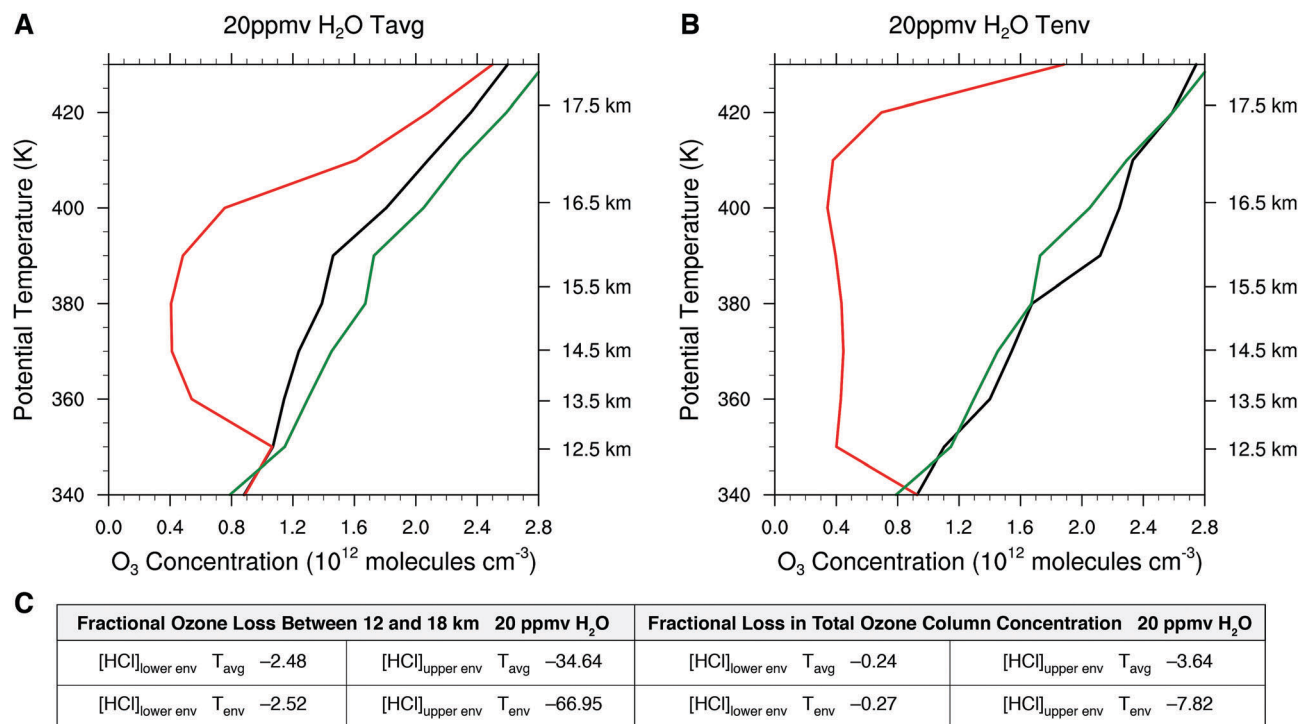
Fig. 14 Panel A displays the impact of the sum of the rate limiting steps for the case of 20 ppmv H 2 O and T_{\text{avg}} for [HCl] lower env displayed in black relative to the unperturbed reference case in green and for [HCl] upper env displayed in red. Panel B displays the same conditions as panel A except for the temperature distribution T_{\text{env}} rather than T_{\text{avg}} . Panel C tabulates the fractional ozone loss between 12 and 18 kilometers and the fraction decrease in the total ozone column density for the temperatures T_{\text{avg}} and T_{\text{env}} relative to the unperturbed reference case in green.
