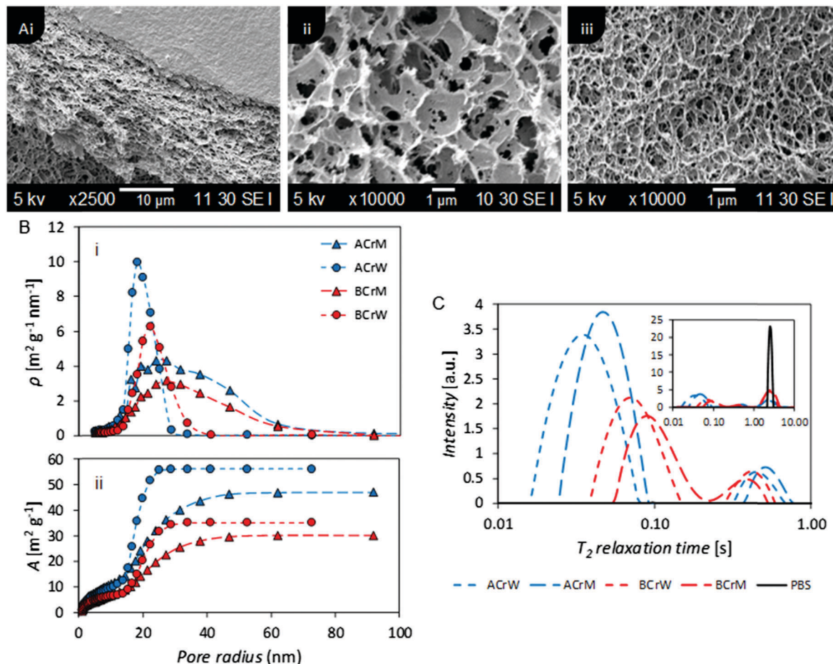
Fig. 2 (A) (i) SEM micrograph of a lyophilised cellulose hydrogel showing the porous structure below a dense skin layer – all hydrogels exhibited this bulk structure, (ii) and (iii) SEM micrographs of ACrM and BCrW samples showing differences in micropore size. (B) Nanometer pore size distribution of hydrogels based on NMR cryoporometry: (i) specific pore surface area density ( \rho ), and (ii) specific cumulative pore surface area. Both choice of cellulose and anti-solvent have an effect on the overall pore structure of the hydrogels in agreement with relaxometry studies. (C) NMR T_2 relaxation distribution curves for regenerated cellulose hydrogels providing relative surface areas for nano- and micropores. Both choice of cellulose and anti-solvent have an effect on the overall pore structure of the hydrogels. Bulk PBS measurement included in inset.
