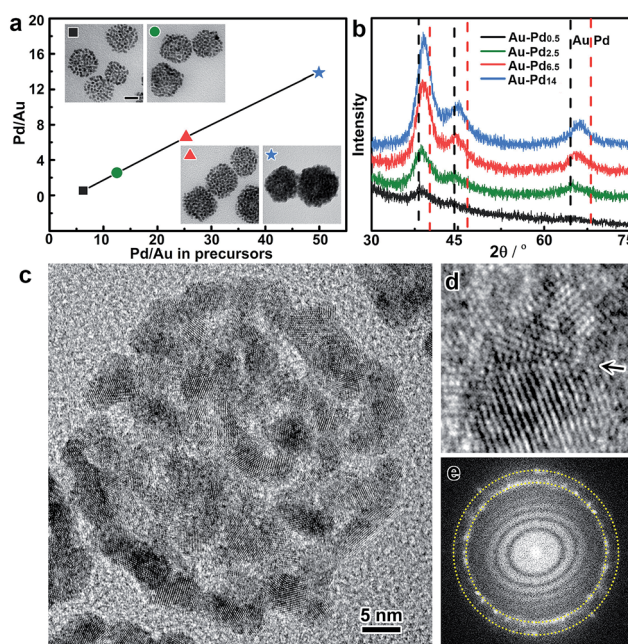
Fig. 3 Compositional and structural analysis of the Au–Pd alloy colloidosomes. (a) The Pd/Au ratio of the Au–Pd alloy colloidosomes as a function of the ratio in the feeding precursor, measured by inductively coupled plasma mass spectrometry (ICP-MS). Inset: TEM images of the Au–Pd alloy colloidosomes with different Pd/Au ratios; scale bar: 20 nm. (b) XRD patterns of the Au–Pd x alloy colloidosomes ( x = 0.5, 2.5, 6.5 and 14 ). The standard peak positions of Au and Pd (111, 200 and 220) are shown for reference. (c) HRTEM image of an individual colloidosome. (d) A defective boundary indicated by an arrow. (e) The corresponding Fourier diffractogram. The dotted lines indicate the {111} and {200} diffraction rings.
