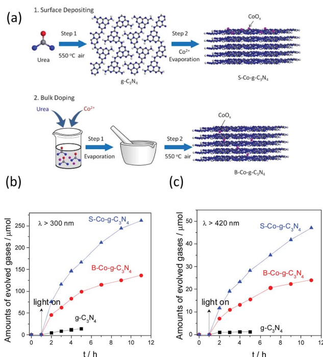
Fig. 11 (a) Schematic illustration of surface modification and bulk doping modification of \text{g-C}_3\text{N}_4 . Photocatalytic water oxidation activities of the \text{g-C}_3\text{N}_4 , \text{B-Co-g-C}_3\text{N}_4 and \text{S-Co-g-C}_3\text{N}_4 samples under (b) UV ( \lambda > 300 \text{ nm} ) and (c) visible light ( \lambda > 420 \text{ nm} ) irradiation. Reprinted with permission from ref. 107. Copyright 2016, American Chemical Society.
