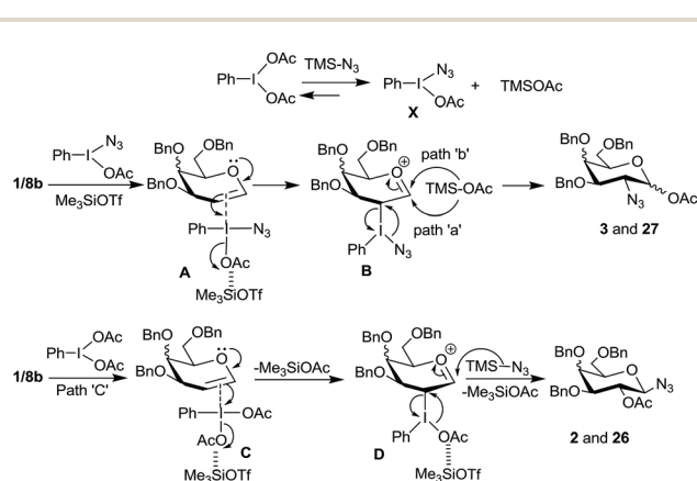
Scheme 7 Proposed mechanisms for the reaction of glycols with PIDA and Me 3 SiN 3 .
