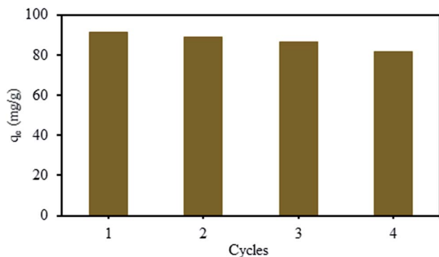
Fig. 12 Recycling of SMGO for the adsorption of Cr(vi). The concentration of SMGO was 1.0 mg L -1 , initial concentration of Cr(vi) = 100 mg L -1 , temperature = 298 K, contact time = 60 min, pH = 3.
