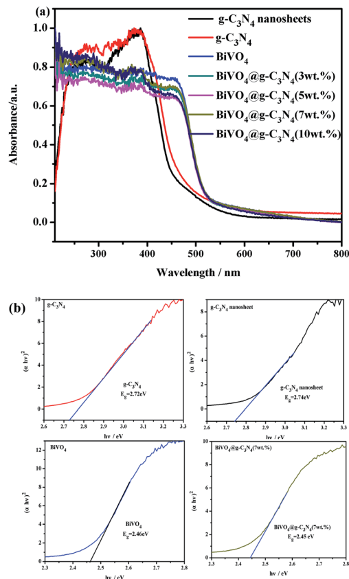
Fig. 6 (a) UV-vis diffuse reflectance spectra of prepared photocatalysts; (b) plot of (\alpha h\nu)^2 vs. energy (h\nu) and band-gap energy of the \text{g-C}_3\text{N}_4 , \text{g-C}_3\text{N}_4 nano-sheet, \text{BiVO}_4 , \text{BiVO}_4/\text{g-C}_3\text{N}_4 samples.
