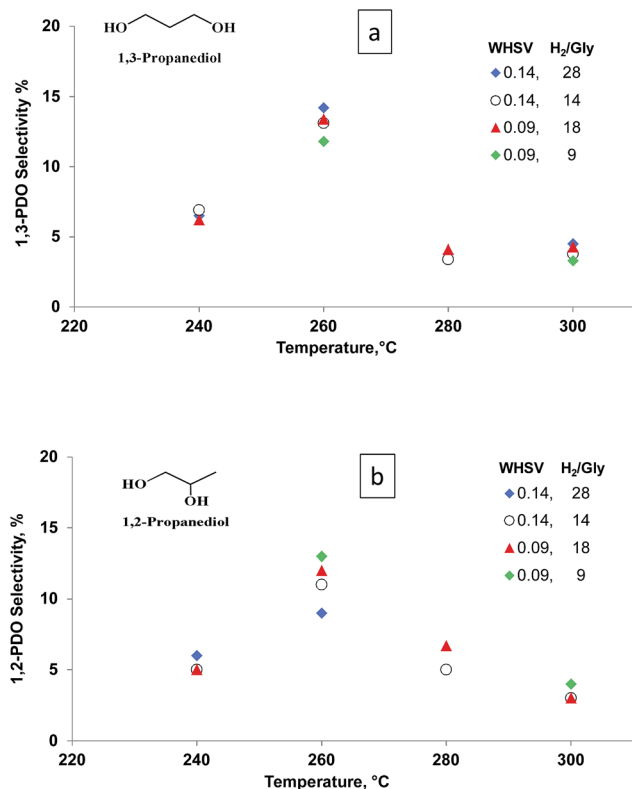
Fig. 5 Selectivity vs. temperature for (a) 1,3-PDO and (b) 1,2-PDO at \text{WHSV} = 0.09 to 0.14 \text{ h}^{-1} , residence time = 0.43 \text{ s} and 0.65 \text{ s} and \text{H}_2/\text{gly} glycerol ratio = 9, 14, 18 and 28.
