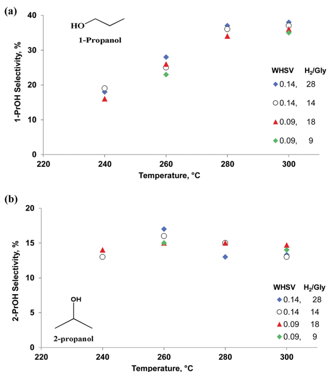
Fig. 6 Selectivity vs. temperature for (a) 1-ProOH and (b) 2-ProOH at \text{WHSV} = 0.09 to 0.14 \text{ h}^{-1} , residence time = 0.43 \text{ s} and 0.65 \text{ s} and \text{H}_2/\text{gly} glycerol ratio = 9, 14, 18 and 28.
