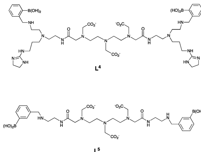
Fig. 12 DTPA-bis amide (DTPA – diethylenetriamine pentaacetic acid) ligands, L 4 and L 5 used in Gd-based MRI contrast agents for sialic acid detection. 5
