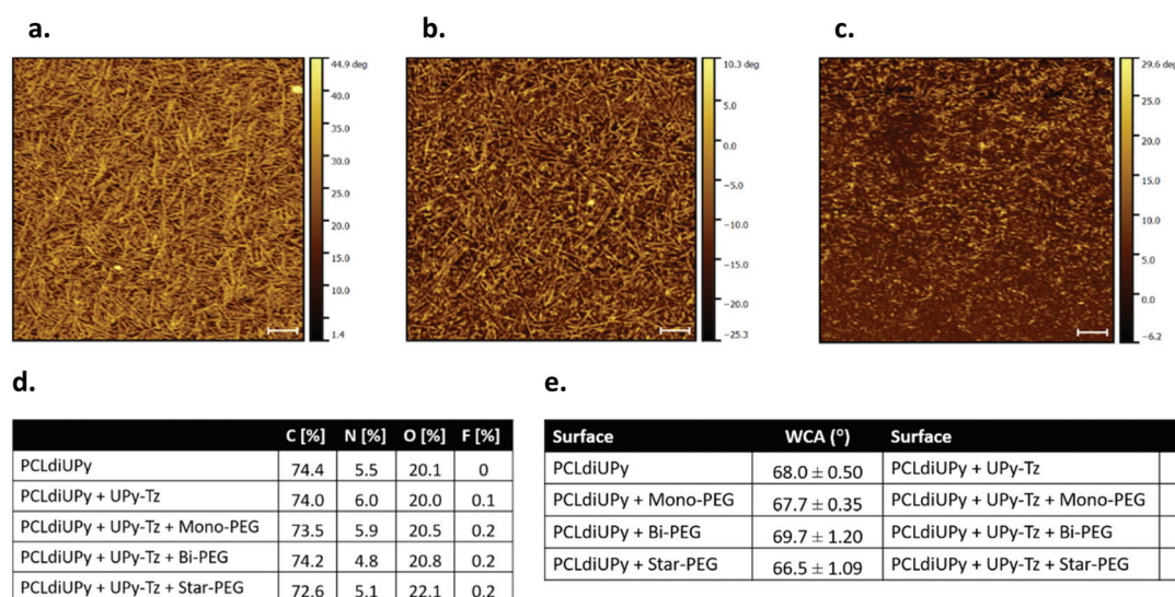
Fig. 2 Surface characterization of the different material films with AFM, XPS and water contact angle. AFM phase micrographs of PCLdiUPy (a), PCLdiUPy with 10 mol% UPy-Tz (b) and after star-PEG-BCN functionalization (c). (d) XPS compositional table of the different surfaces and (e) water contact angles of the respective surfaces. Five measurements were performed per surface and standard deviations are plotted.
