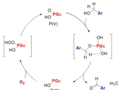
Scheme 20 Proposed mechanism for aerobic oxidation of benzyl alcohol by P-doped carbon. Reproduced from ref. 96 with permission from American Chemical Society, copyright 2017.
