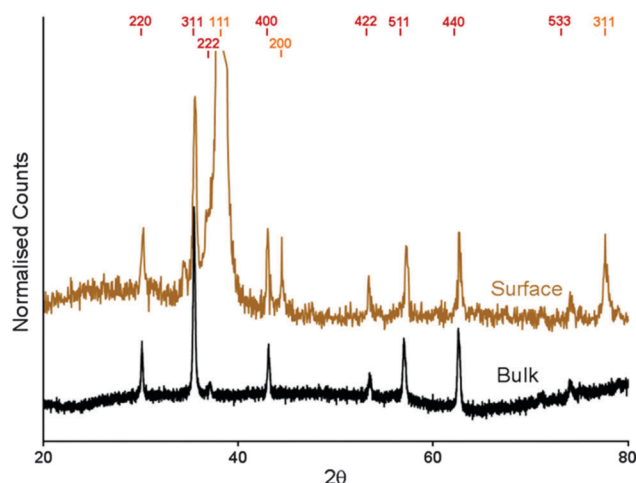
Fig. 4 XRD data recorded for the MNPs biomaterialised by Mms6 onto gold (gold) and of the control particles that form in solution (black) during a POFHK reaction. The expected peak positions for magnetite (red) and gold (gold) are highlighted.
