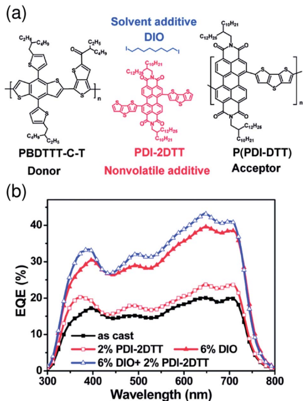
Fig. 12 (a) Chemical structures of the PBDDTTT-C-T donor, P(DI-DTT) acceptor, PDI-2DTT, and DIO. (b) EQE spectra of PBDDTTT-C-T/P(DI-DTT) blend solar cells without or with additives under AM 1.5G solar simulator illumination at 100 mW cm -2 . Reproduced with permission from (ref. 56). Copyright 2013, The Royal Society of Chemistry.
