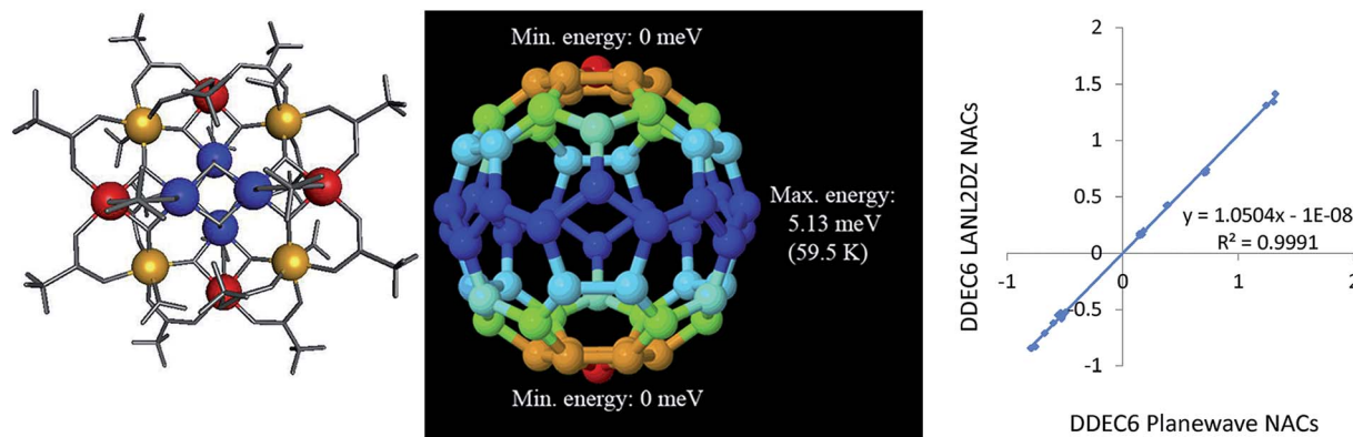
Fig. 9 Left: Atomic structure of \text{Mn}_{12} -acetate single molecule magnet. Mn type 1 (blue), Mn type 2 (red), Mn type 3 (yellow). In the minimum energy conformations, the Mn ASM vectors are perpendicular to the plane of the page. Middle: Computed spin-orbit coupling potential energy surface. Right: Comparison of DDEC6 NACs computed with LANL2DZ and planewave basis sets.
