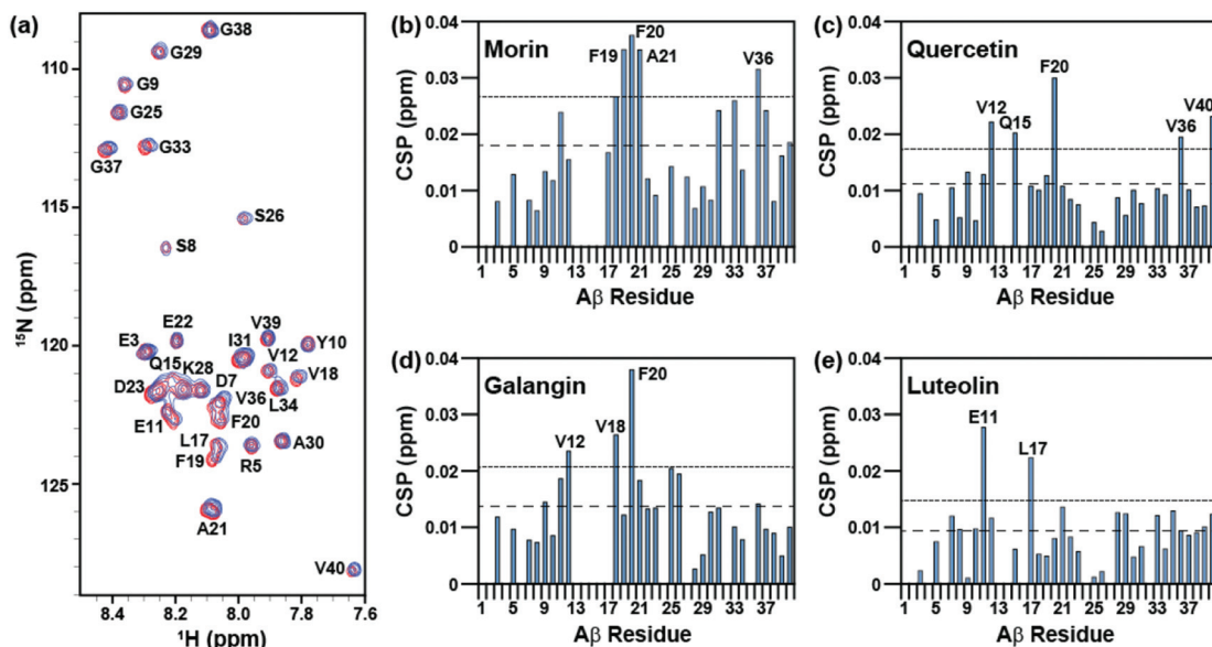
Fig. 5 \text{A}\beta interaction of the flavonoids, monitored by 2D SOFAST-HMQC NMR. NMR spectra were recorded as (a) morin was titrated into a solution of ^{15}\text{N} -labeled \text{A}\beta_{40} from 0 (red spectra) and 10 (blue spectra) equiv. of the flavonoids. The chemical shift perturbation (CSP) was calculated for each residue upon the titration of (b) morin, (c) quercetin, (d) galangin, and (e) luteolin in order to investigate their potential interaction with \text{A}\beta . The average chemical shift (dashed line) plus standard deviation (dotted line) were plotted for the reference. CSP values which exceed the sum of the average CSP and the standard deviation are indicative of noticeable interactions. Conditions: [\text{A}\beta_{40}] = 80 \mu\text{M} ; [\text{flavonoids}] = 0\text{--}800 \mu\text{M} ; 20 mM \text{PO}_4 , pH 7.4, 50 mM NaCl; 7% \text{D}_2\text{O} (v/v); 10 °C.
