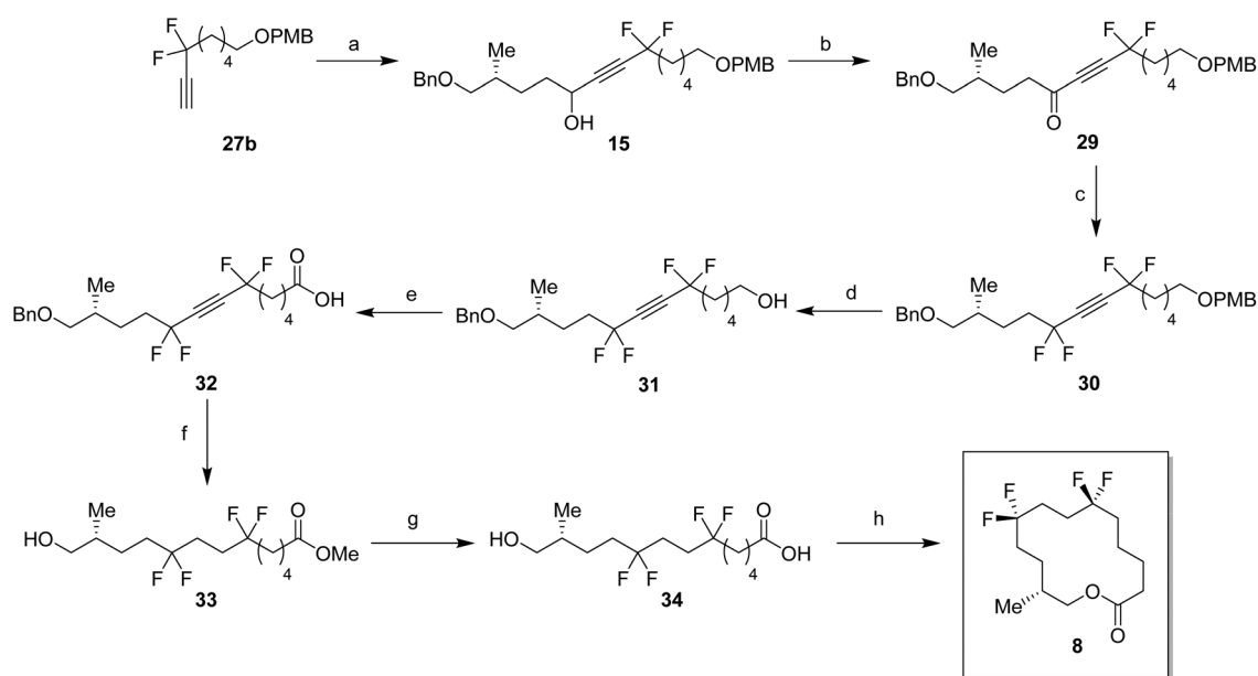
Scheme 4 Synthesis of musk lactone 8 . Reagents and conditions: (a) (i) n\text{BuLi} , THF, -78\text{ }^\circ\text{C} , 30 min. (ii) Aldehyde 12 , THF, -78\text{ }^\circ\text{C} –r.t., 20 h, 61%; (b) DMP, DCM, r.t., 2 h, 89%; (c) DAST, 50 °C, 18 h, 71%; (d) DDQ, DCM, \text{H}_2\text{O} , r.t., 2 h, 78%; (e) BAIB, TEMPO, \text{CH}_3\text{CN} , \text{H}_2\text{O} , r.t., 7 h, 58%; (f) palladium on carbon (10 wt%), \text{H}_2 , MeOH, r.t., 18 h, 65%; (g) LiOH, THF, \text{H}_2\text{O} , r.t., 3 h, 94%; (h) 2,4,6-trichlorobenzoyl chloride, \text{NEt}_3 , THF, r.t., 2.5 h. (ii) 4-DMAP, toluene, r.t., 3.5 h, 54%.
