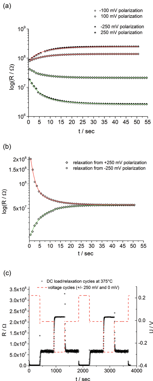
Fig. 6 A finite time is required to reach a steady state resistance under an applied bias voltage. This is shown in (a) for a 150 nm STO film at 375^\circ\text{C} ( T_{\text{set}} ) and \pm 100 mV and \pm 250 mV, respectively. By switching off the voltage, a relaxation process takes place. In (b) the relaxation of the resistance probed by a small DC voltage ( \pm 5 mV) after polarization by \pm 250 mV at 375^\circ\text{C} ( T_{\text{set}} ) is shown. (c) Various cycles with positive and negative voltages show the reproducibility of the polarization and relaxation processes.
