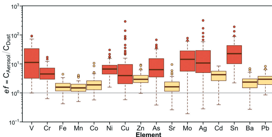
Fig. 3 Ratios of the concentration of metals in aerosolized samples over bulk dust, representing the overall enrichment of metals in aerosolized samples (or “aerosol enrichment factor”, ef). A horizontal line was added to the ratio of 1 to represent the hypothetical point in which there would be no significant difference between bulk and aerosolized samples. An ef greater than one signifies that aerosolized samples contain a relatively higher concentration of said metal than bulk dust samples, which may indicate that said metal is more likely to be present in particles smaller than 2.5 \mu\text{m} . Groups with average ef > 5 are highlighted in red (darker shade).
