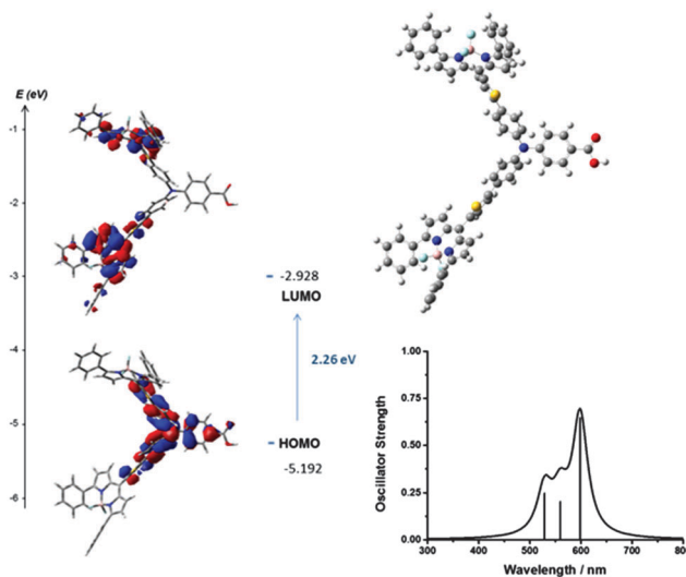
Fig. 7 Optimised geometry and calculated principle energy transitions for 5 determined by DFT and TD-DFT (in dichloromethane solvent) using B3LYP/6-31G(d).
