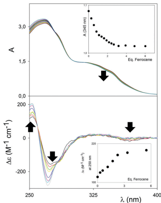
Fig. 2 Top: UV titration of metal-linked macrocycle (RR)-7 ( 2.5 \times 10^{-5} M) with ferrocene in MeCN at 25^\circ\text{C} . Inset: Titration profile vs. ferrocene added equivalents at 345 nm. Bottom: CD titration of macrocycle (RR)-7 ( 1 \times 10^{-5} M) with ferrocene in MeCN at 25^\circ\text{C} . Inset: Titration profile vs. ferrocene added equivalents at 250 nm.
