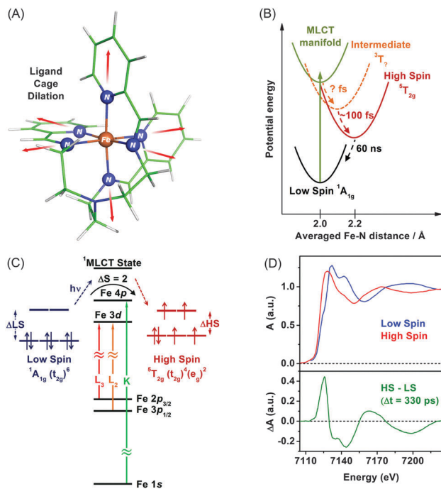
Fig. 2 (A) Molecular structure of [Fe(tren(py) 3 )] 2+ . The changes of metal–ligand bonds associated with the spin transition are indicated by arrows. (B) Simplified energy levels involved in intersystem crossing after optical excitation to the metal-to-ligand charge-transfer state. (C) Schematic of orbitals associated with X-ray absorption spectroscopic measurements at multiple X-ray absorption edges. (D) (lower panel) Transient difference XAS spectrum (red) of [Fe(tren(py) 3 )] 2+ measured at the time delay of 330 ps. (Upper panel) The steady-state XAS spectra of high-spin and low-spin Fe complexes is plotted together.
