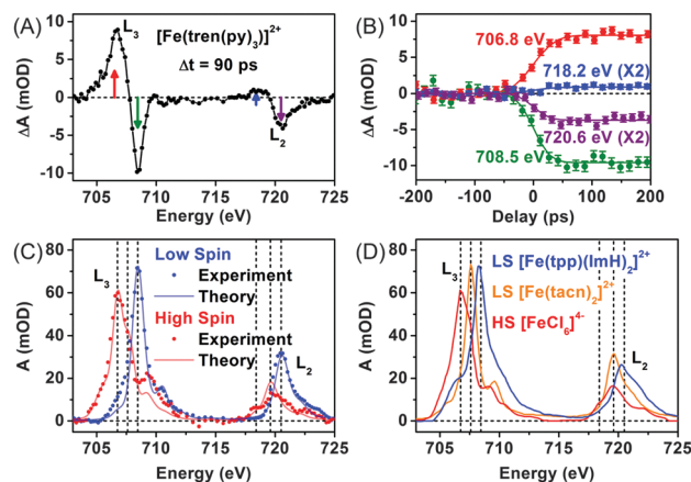
Fig. 3 (A) TRXAS spectrum at 90 ps for [Fe(tren(py) 3 )] 2+ SCO processes at Fe L 2,3 -edges. (B) Temporal changes of the TRXAS signal at selected energies indicated with colored arrows in (A). (C) L-edge spectra of the low-spin ground state (blue points) and the transient high-spin state at 90 ps delay (red points). The high-spin spectrum was reconstructed from the differential absorption spectrum shown in (A). For comparison with the experiment, theoretical spectra were obtained from charge transfer multiplet calculations (colored lines). (D) Rescaled L-edge spectra of three crystalline compounds: [Fe(tpp)(ImH) 2 ] 2+ , [Fe(tacn) 2 ] 2+ , and [FeCl 6 ] 4- .
