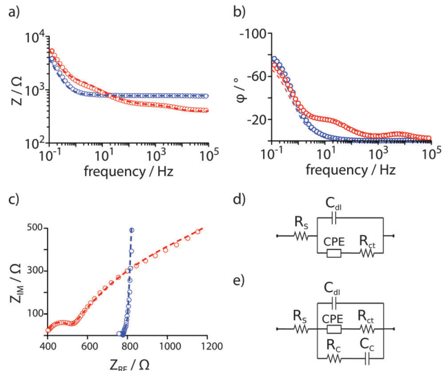
Fig. 2 EIS of electrodeposited PEDOT:PSS in the absence (blue) and presence (red) of a confluent layer of MDCK cells in supplemented cell culture medium. (a) Impedance Z and (b) phase angle \varphi presented in Bode plots. (c) A Nyquist plot shows Z_{RE} and Z_{IM} as polar coordinates, Z(\omega) = Z_{IM} \sin \varphi^{-1} = Z_{RE} \cos \varphi^{-1} , \omega = 2\pi f . Data were fitted with an equivalent circuit model adapted from Richardson-Burns et al. 12 Experimental data = open circles, fitted data = dashed lines. (d) The equivalent circuit used to fit EIS data in supplemented cell culture medium only. (e) The extended equivalent circuit model used to fit EIS data arising from a confluent monolayer of cells on the PEDOT:PSS PAS electrodes.
