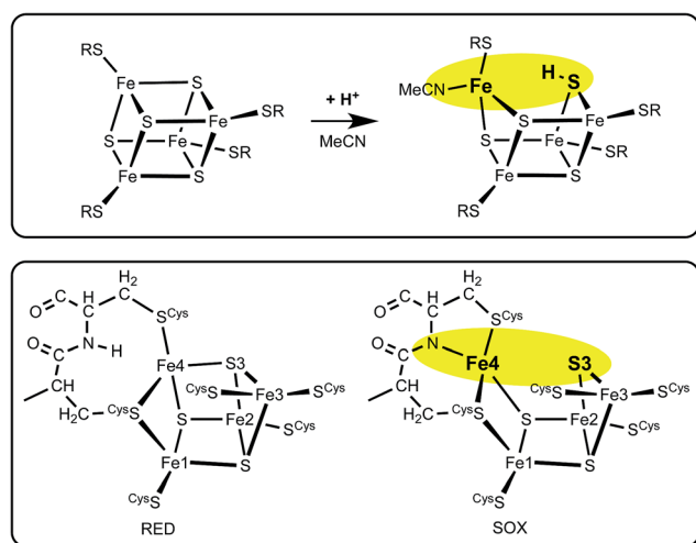
Fig. 3 The similarity between the change on protonation of [\text{Fe}_4\text{S}_4(\text{SR})_4]^{2-} in acetonitrile (upper panel), and the structural change RED → SOX in the proximal cluster (lower panel).
