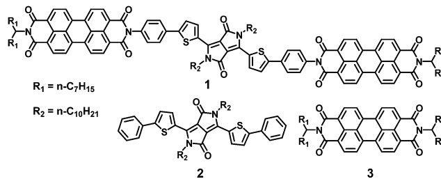
Chart 1 Molecules referenced in this paper.
