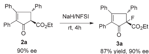
Scheme 3 Product transformation.
