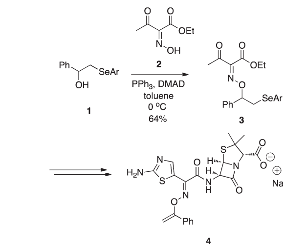
Scheme 2 Oximes as oxygen pronucleophiles in the Mitsunobu reaction.
