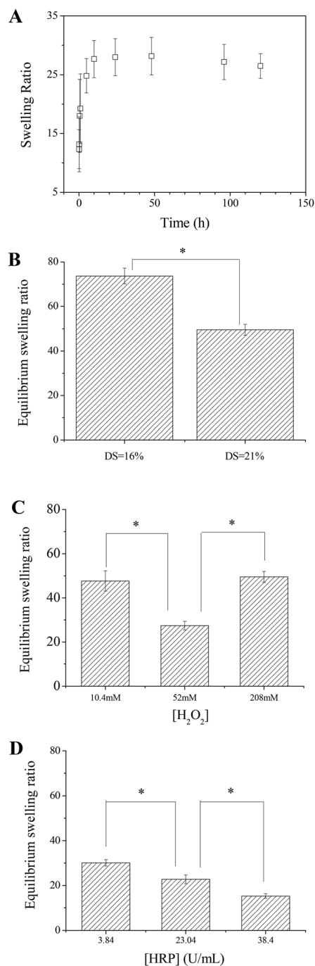
Fig. 5 (A) Swelling kinetics of an Alg–DA hydrogel in PBS. T = 37 °C. Gel parameters: [polymer] = 4 wt%, DS = 21\% , [HRP] = 23.04 U mL -1 , [H_2O_2] = 52 mM. (B) Equilibrium swelling ratios of Alg–DA hydrogels as a function of DS. Other parameters: [polymer] = 4 wt%, [HRP] = 23.04 U mL -1 , [H_2O_2] = 208 mM. (C) Equilibrium swelling ratios of Alg–DA hydrogels as a function of [H_2O_2] . Other parameters: [polymer] = 4 wt%, DS = 21\% , [HRP] = 23.04 U mL -1 . (D) Equilibrium swelling ratios of Alg–DA hydrogels as a function of [HRP] . Other parameters: [polymer] = 4.0 wt%, DS = 21\% , [H_2O_2] = 52.0 mM. * indicates statistical significance at the 0.05 level.
