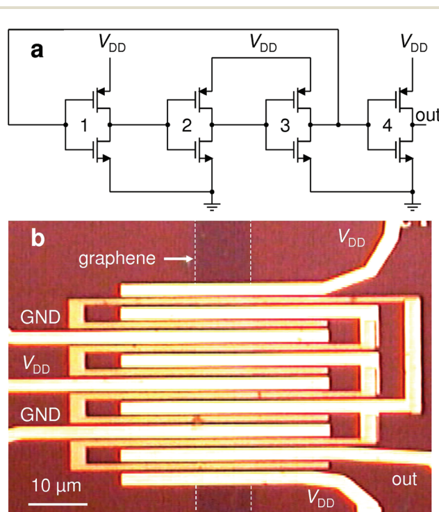
Fig. 63 Integrated GRO. (a) Circuit diagram of a three-stage RO. The RO comprises three inverters (1–3) cascaded in a loop with a fourth inverter (4) decoupling the RO from the measurement equipment connected to the output (out). (b) Optical microscope image of a RO with gate length L = 1 \mu\text{m} integrated on a CVD graphene channel. The drain contacts of inverters 1–3 (Au) overlap with the gate contacts (Au/Ti/Au) in order to form internal connections between the inverters. GND = ground. Adapted from ref. 1102.
