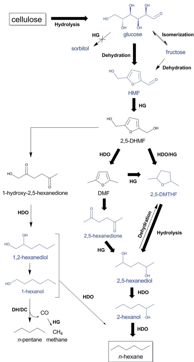
Scheme 3 Proposed reaction pathways from cellulose to n -hexane and n -pentane through HMF with TSA and htTSA(2)Ru/C, partially based on Liu et al. , 88 Alamillo et al. , 67 Li et al. 60 and Yang et al. 92 Intermediates tested in this study are indicated in blue. The most selective reaction pathway from cellulose to n -hexane is indicated with bold arrows. HDO, hydrodeoxygenation; HG, hydrogenation; DH/DC, dehydrogenation/decarbonylation.
