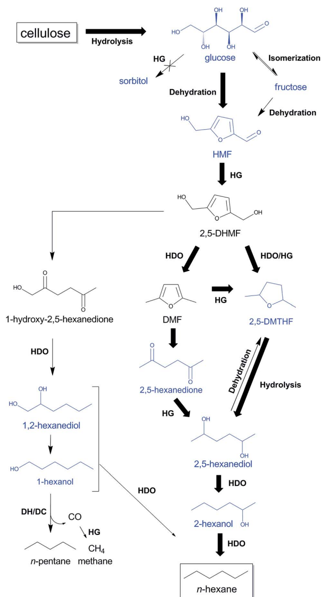
Scheme 3 Proposed reaction pathways from cellulose to n -hexane and n -pentane through HMF with TSA and htTSA(2)Ru/C, partially based on Liu et al. , 68 Alamillo et al. , 67 Li et al. 60 and Yang et al. 92 Intermediates tested in this study are indicated in blue. The most selective reaction pathway from cellulose to n -hexane is indicated with bold arrows. HDO, hydrodeoxygenation; HG, hydrogenation; DH/DC, dehydrogenation/decarbonylation.
