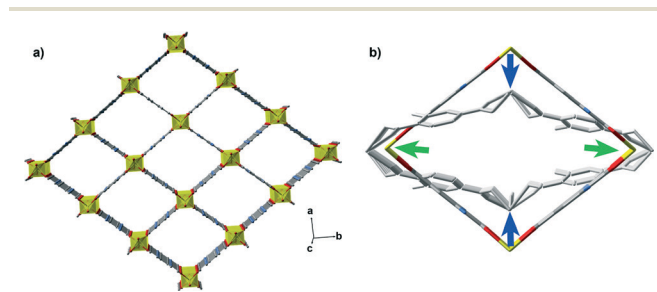
Fig. 1 (a) The MIL-53 framework in its lp configuration, with a wine-rack framework topology and (b) the expected NLC behaviour.
