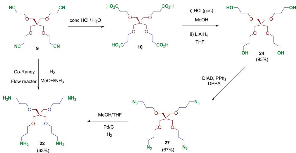
Scheme 8 Synthesis of tetrapodal polyamine (22) and polyazide (27) scaffolds.
