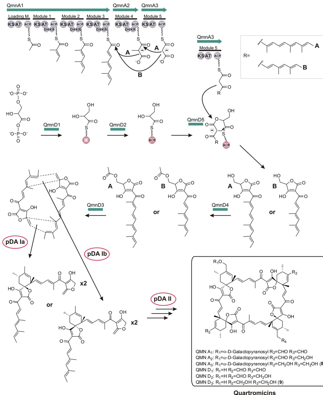
Fig. 11 Model for quartromicin biosynthesis. The multienzyme polyketide synthase complex (QmnA1-3) synthesizes two different linear polyketide precursor molecules by mechanistic module skipping. Each single precursor unit is then tethered to a preactivated and ACP-coupled C 3 -unit, derived from 1,3-bisphosphoglycerate. Tetronic acid maturation steps depicted in this figure were recently elucidated (QmnD1-5: protein set encoded by the conserved "glycerate utilization operon"). Multiple intermolecular Diels–Alder reactions between the exocyclic methylene group of the tetronic acid moiety of one precursor and a pair of conjugated double bonds in the tail-region of another linear polyketide are proposed to take place, thereby generating the quartromicin macrocycle in a head-to-tail fashion (pDA = postulated Diels–Alder reaction). The exact sequence of all fusion events remains elusive. Further decoration reactions on the macrocyclic structure produce quartromicin and its derivatives.
