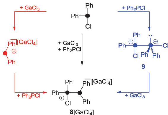
Scheme 1 Synthesis of 8[GaCl_4] by the reaction of Ph_2PCL and GaCl_3 in 2 : 1 stoichiometry and possible reaction sequences giving 8[GaCl_4] either via free Ph_2P^+ -phosphonium ion (red) or zwitterion 9 (blue).
