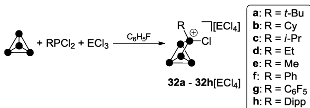
Scheme 8 Preparation of compounds 32a-h[ECl_4] from P_4 , RPCl_2 and ECl_3 ( E = Ga, Al ; R = \text{alkyl, aryl} ) in fluorobenzene.
