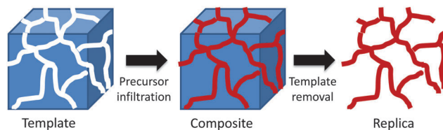
Fig. 5 A schematic representation of the nanocasting pathway using a 3D-interconnected hard template.
