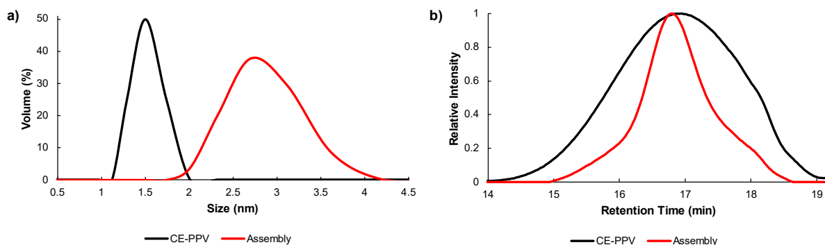
Figure 3. (a) DLS in 1:1 \text{CHCl}_3/\text{CH}_3\text{CN} and (b) GPC characterization in THF, against linear PS standards, of homopolymer CE-PPV ( 13b ) (black) and the supramolecular bottlebrush CE-PPV-PS-DBA ^+ (red).
