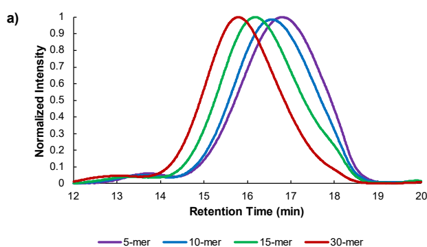
Figure 1. a) Molecular weight distribution of polymers 13a-d (GPC in THF). (b) Dependence of M_n as measured by GPC of polymers 13a-d on the [M]/[I] ratio. Here, 13a , n = 5 , 13b , n = 10 , 13c , n = 15 , and 13d , n = 30 . Dispersity values of the respective polymers are denoted in the plot.
