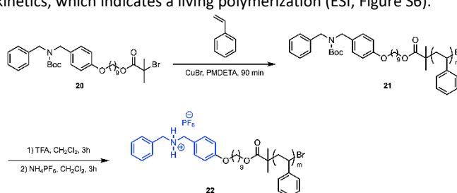
Scheme 5. Synthesis of telechelic PS-DBA + , 22 .
