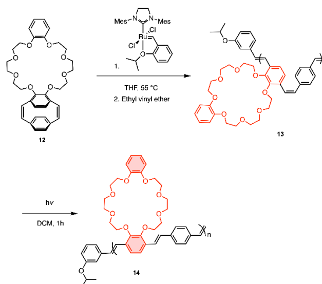
Scheme 4. ROMP of CE- p Cpd, 12 , and photo-isomerization at 395 nm.
