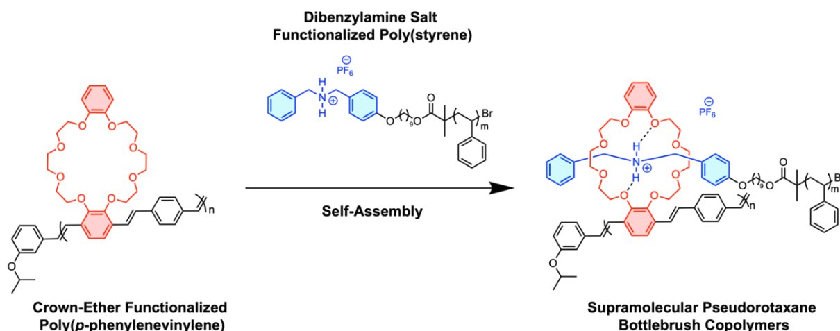
Scheme 2. Synthesis of supramolecular bottlebrush copolymers based on host-guest interactions between crown-ether functionalized poly( p -phenylenevinylene) and dibenzyl amine end-functionalized poly(styrene).
