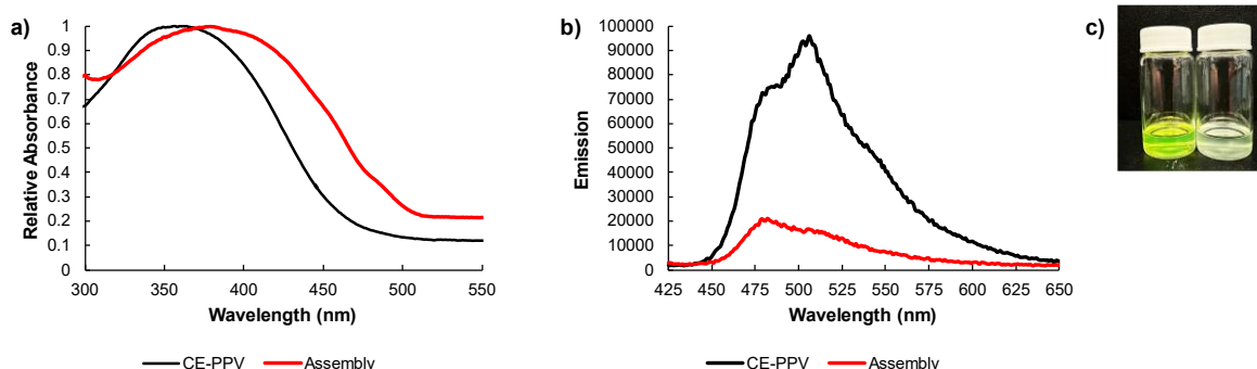
Figure 4. a) Absorbance spectra and b) Emission spectra of homopolymer CE-PPV ( 13b ) (black) and the supramolecular bottlebrush CE-PPV-PS-DBA + (red). c) The CE-PPV has strong fluorescence (left) and the bottlebrush has quenched fluorescence (right).
