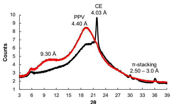
Figure 5. WAXS diffractograms corresponding to homopolymer CE-PPV ( 13b ) (black) and the supramolecular bottlebrush CE-PPV-PS-DBA + (red).
