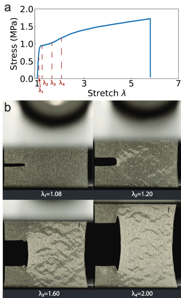
Fig. 3 (a) Representative stress-stretch behavior of notched PDUO-GF composites with 5 vol.% fibers. (b) Optical images of the deformation of the sample at indicated stretch levels (video of the test can be found in supplemental movie S1).
