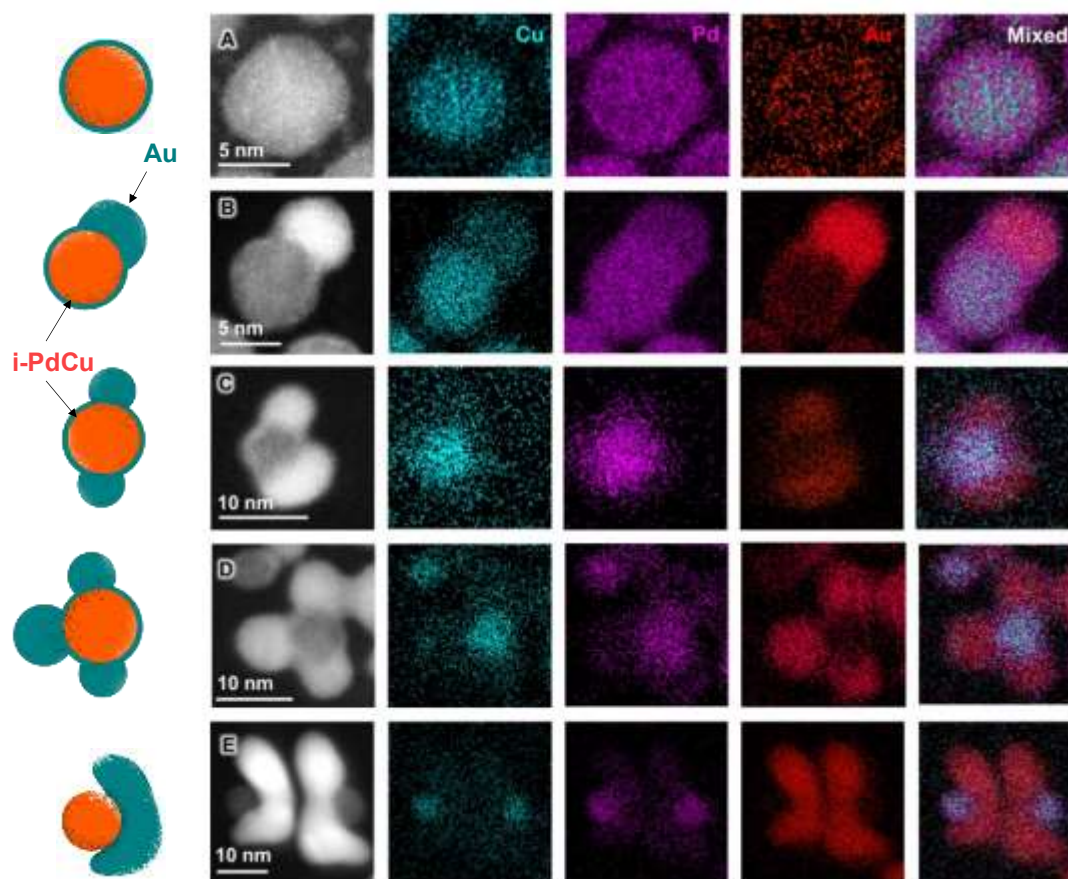
Figure 3. (Left-right) Models, HAADF-STEM images, and STEM-EDS maps of products from GR of i-PdCu NPs titrated with A) 1.5 mL (no domain core@shell i-PdCu@Au), B) 4.5 mL (one domain), C) 9 mL (two domains), D) 9 mL (three domains), and E) 25 mL (boat-shaped) of 0.1mM \text{AuCl}_2^- solution.
