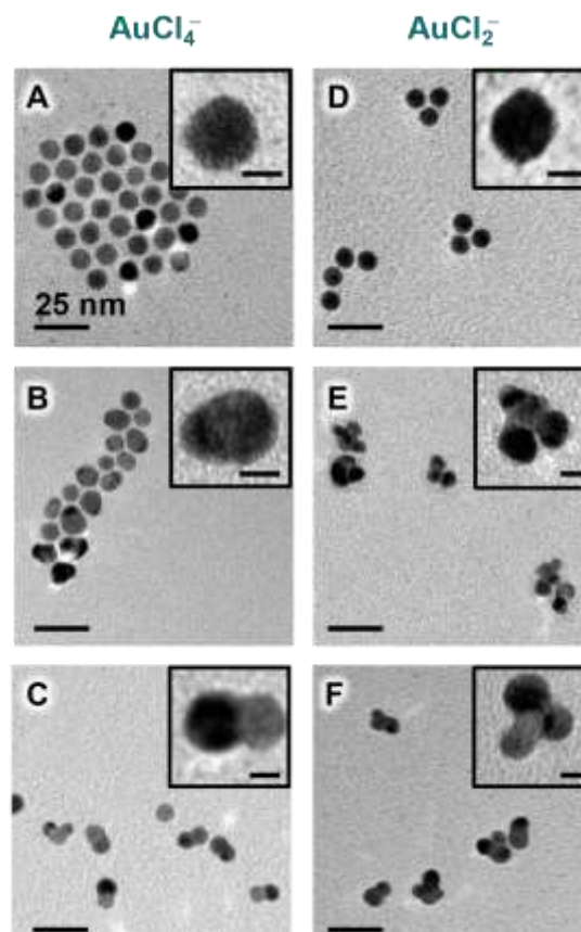
Figure 1. TEM images of products obtained from GR between i-PdCu NPs and A) 0.5, B) 1.5, and C) 3 mL of 0.1 mM \text{AuCl}_4^- or D) 1.5, E) 4.5, and F) 9 mL of 0.1 mM \text{AuCl}_2^- . Scale bars = 25 nm for all (inset scale bars = 5 nm).
