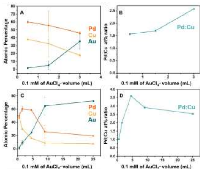
Figure 4. (A–C) Plot of titrant volume vs. atomic percentages showing the evolution of atomic percentage determined by SEM-EDS of Pd, Cu, and Au, (B–D) Plot of titrant volume vs Pd:Cu atomic percentage ratio showing the evolution of Pd, Cu ratio in i-PdCu system.
