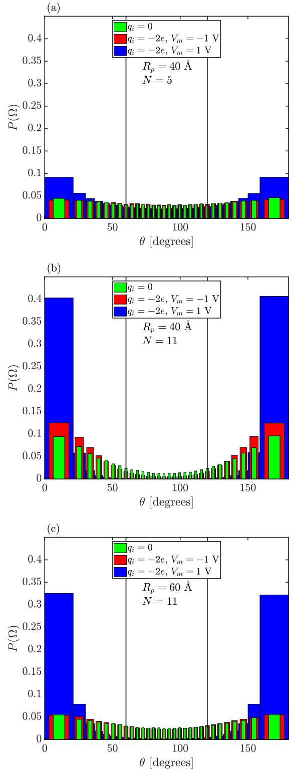
FIG. 4. The probability of the capsule's orientation angle \theta while in the pore (computed using equal solid angles \Omega ), P(\Omega) , for q_i = -2e at V_m = \pm 1 V, and q_i = 0 , in the following cases: (a) R_p = 40 Å, N = 5 ( L_c = 30 Å), (b) R_p = 40 Å, N = 11 ( L_c = 60 Å), (c) R_p = 60 Å, N = 11 ( L_c = 60 Å). The solid lines indicate angles \theta_{up} = 60^\circ and \theta_{down} = 120^\circ (see Sec. III C).
