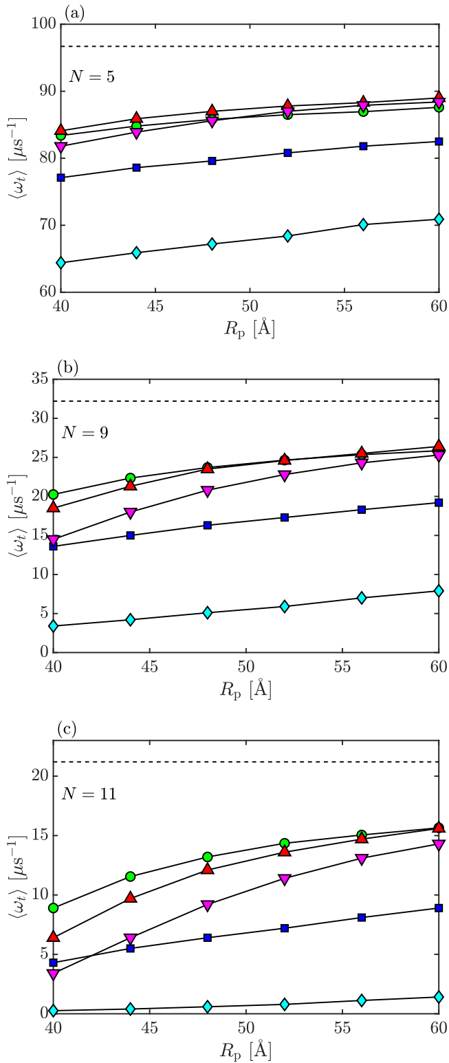
FIG. 8. The capsule's tumbling rate, \langle \omega_t \rangle , for R_p = 40 \text{ \AA} to 60 \text{ \AA} for parameters: ( \nabla ) V_m = -1 \text{ V} , q_i = -2e ; ( \triangle ) V_m = -1 \text{ V} , q_i = -1e ; ( \circ ) q_i = 0 ; ( \square ) V_m = 1 \text{ V} , q_i = -1e ; ( \diamond ) V_m = 1 \text{ V} , q_i = -2e ; Dashed line is for q_i = 0 in free space (outside of the pore). The capsule lengths studied include (a) N = 5 , (b) N = 9 , and (c) N = 11 .
