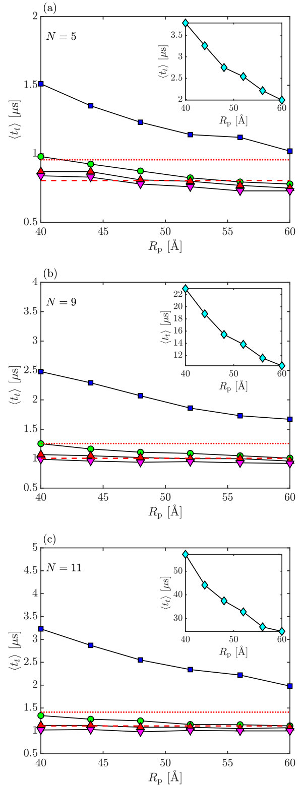
FIG. 6. The capsule's average translocation time, \langle t_t \rangle vs. nanopore radius R_p for (a) N = 5 , (b) N = 9 , and (c) N = 11 : ( \nabla ) V_m = -1 \text{ V} , q_i = -2e ; ( \Delta ) V_m = -1 \text{ V} , q_i = -1e ; ( \circ ) q_i = 0 ; ( \square ) V_m = 1 \text{ V} , q_i = -1e ; ( \diamond ) V_m = 1 \text{ V} , q_i = -2e (inset). The horizontal dashed and dotted line correspond to free diffusion times L^2 \xi_{\parallel} / 6k_b T and L^2 \xi_{\perp} / 6k_b T , respectively.
