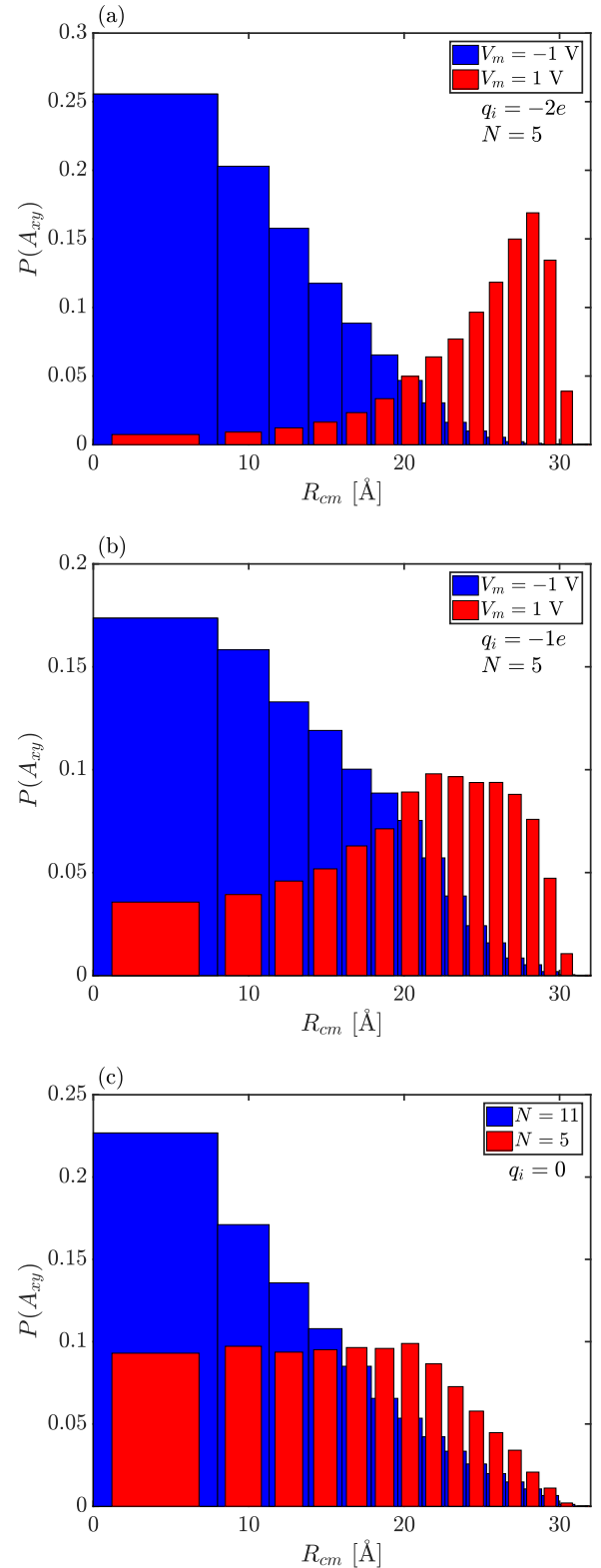
FIG. 5. The probability of the capsule's center of mass location P(A_{xy}) in the radial direction, R_{cm} , while inside the pore (using computed equal area A_{xy} concentric circles) for pore radius R_p = 40 Å. (a) q_i = -2e ( N = 5 ), V_m = \pm 1 V, (b) q_i = -1e ( N = 5 ), V_m = \pm 1 V, (c) q_i = 0 , N = 5 and N = 11 .
