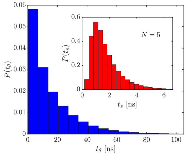
FIG. 7. Histograms of total tumbling times, t_\theta , and (inset) only successful tumbling attempts, t_s , for N = 5 , q_i = -2e capsules in a R_p = 40 \text{ \AA} , V_m = 1 \text{ V} pore. The averages \langle t_\theta \rangle and \langle t_s \rangle extracted from the histograms are 15.5 and 1.7 ns, respectively.
