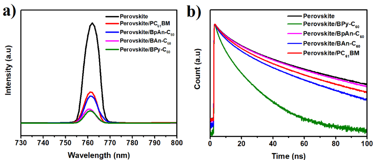
Figure 6: a) SS and b) TRPL for devices constructed as MAPbI 3 /fullerene derivatives.
