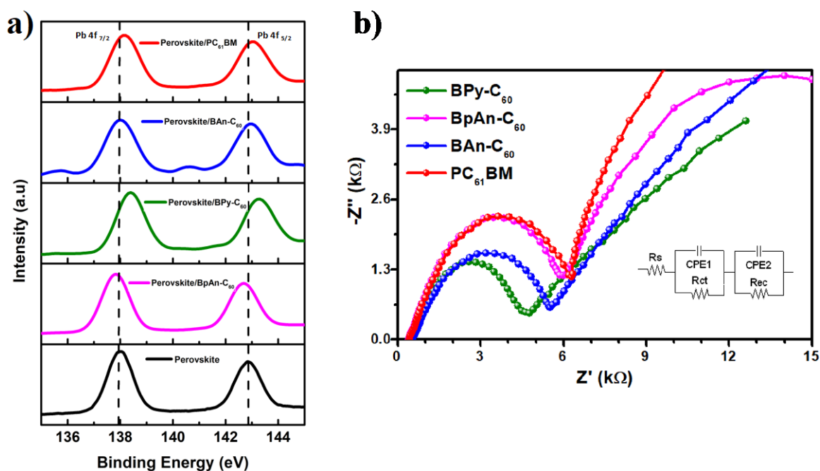
Figure 7: a) XPS measurements of the Pb 4f region for MAPbI 3 /fullerene films and b) EIS studies for devices fabricated with the as-synthesized fullerene derivatives.
