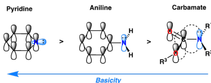
Figure 1: Orbital representation of pyridine, aniline and carbamate.
