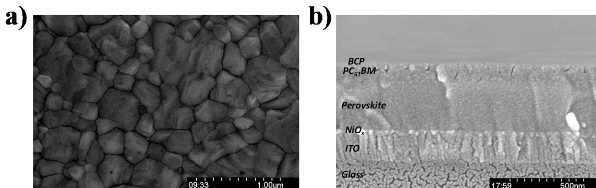
Figure 4: a) SEM of the perovskite surface, b) Cross-section SEM to the general device architecture.
