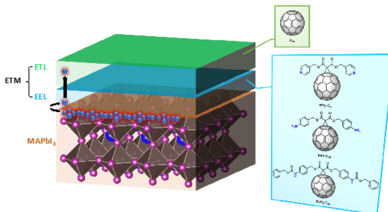
Figure 2: a) Device structure with the fullerene C 60 , BPy-C 60 , BAn-C 60 and BpAn-C 60 used as ETM, EEL and ETL.
