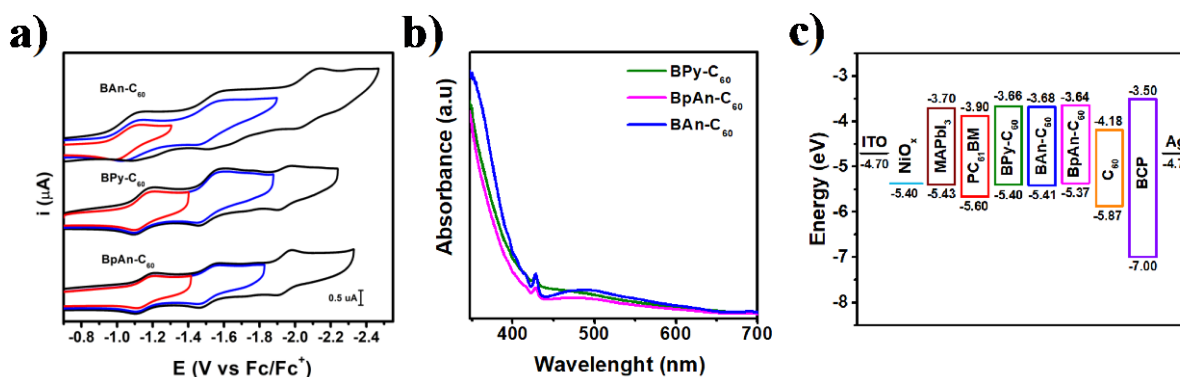
Figure 3: a) Cyclic voltammetry, b) UV-Vis and c) energy level diagram for the compounds BPy-C 60 , BAn-C 60 and BpAn-C 60 .
