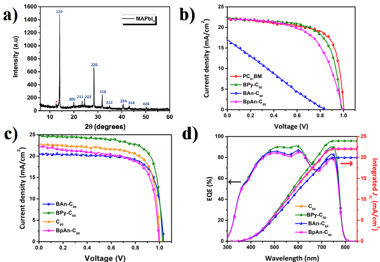
Figure 5: a) XRD characterization of the perovskite, b) J - V curves of devices with the new compounds used as ETM, c) J - V curves and d) EQE for the devices with the new compounds used as EEL.
