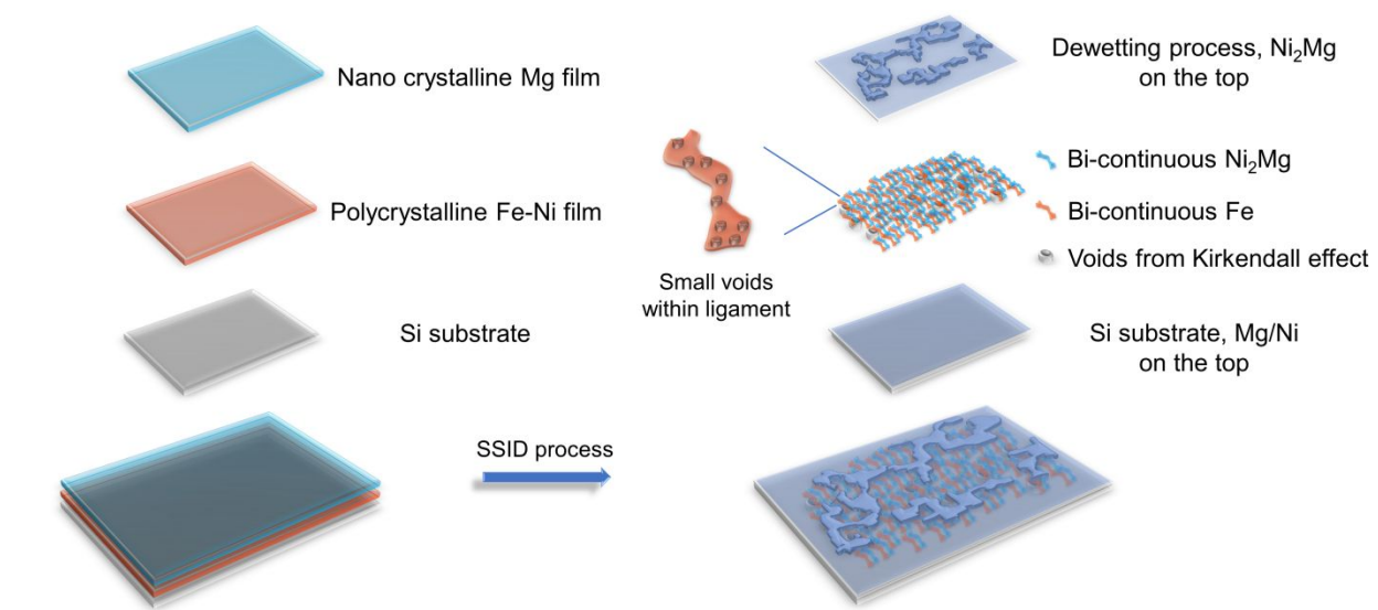
Fig. 5 Schematic of morphological evolution of thin-film-SSID in Fe-Ni/Mg system.
