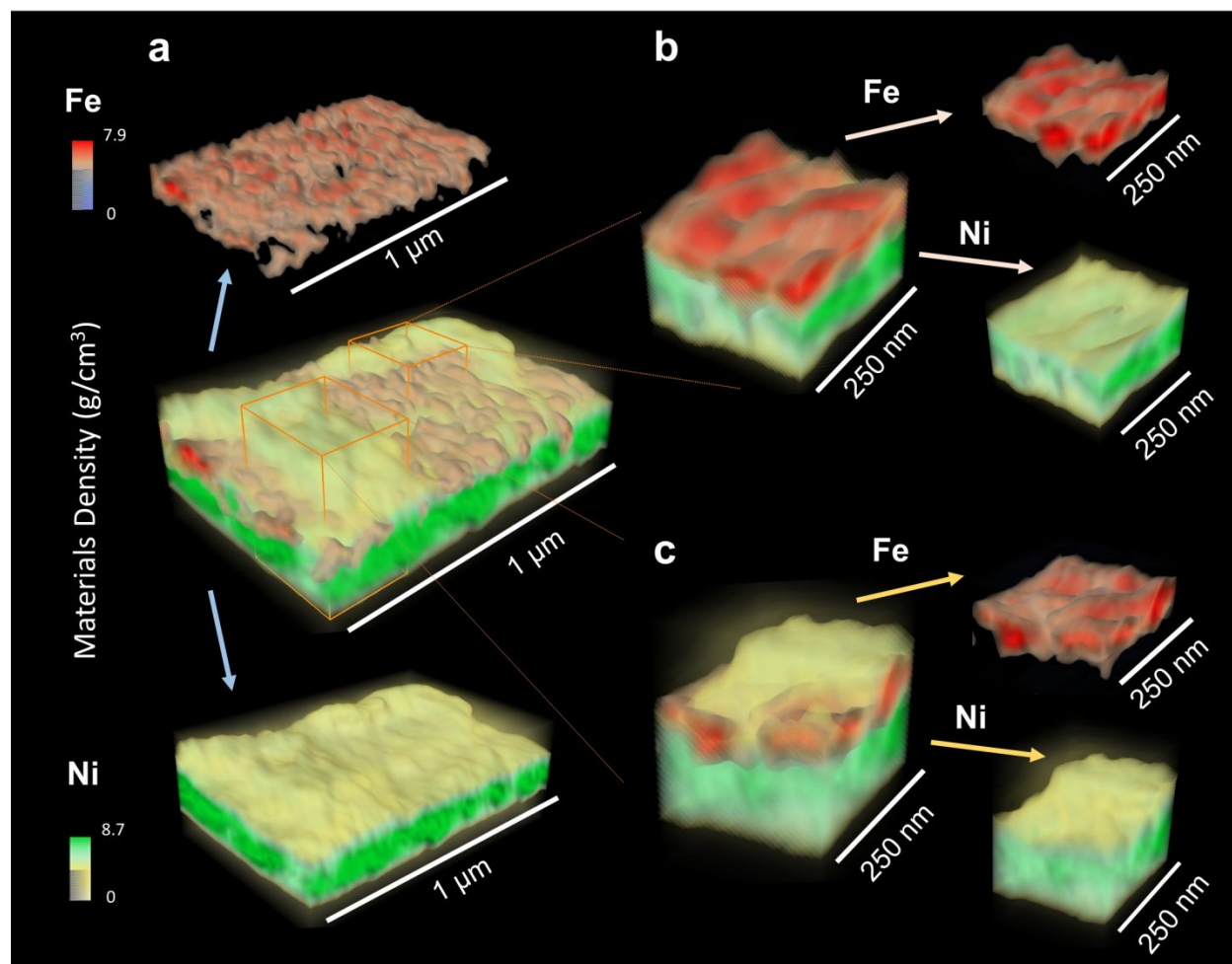
Fig. 2 3D XRF nano-tomography of Fe-Ni thin film dealloyed with Mg (S100-D2) by SSID at 460°C for 30 min from Hard-X-ray Nano-probe at NSLS-II. a Representative volume shows Fe and Ni spatial distributions b-c Cropped sub-volumes to compare structures: b from the region without Ni agglomeration c from the region with Ni film agglomeration. Supplementary Video 1 based on the 3D XRF nano-tomography can be found in supporting information online. Color scale corresponds to the materials density ( \text{g}/\text{cm}^3 )
