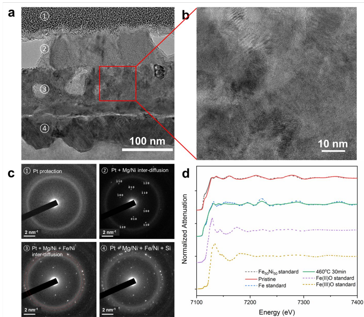
Fig. 4 a TEM image of Fe-Ni films dealloyed with Mg under 460°C for 30 min (S100-D1). b Zoom-in view of TEM image on separate Fe and Ni-Mg inter-diffusion layer c The SAEDs were collected from the top to the bottom, including Pt protection layer, Pt with inter-diffuse Mg-Ni, Pt with Mg-Ni and inter-diffuse Fe-Ni layer, and whole films with Si substrate. d XANES was collected on Fe, Fe(II)O, Fe(III)O, FeNi (50-50 at.%) standard powder, pristine (S100-P2) and sample dealloyed at 460°C for 30 min (S100-D3).
