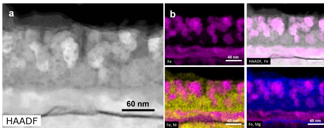
Fig. 1 STEM analysis of Fe-Ni films dealloyed by Mg film at 460°C for 30 min (S100-D1) showing the morphology and composition at the dealloying front, indicating formation of Fe and Ni x Mg phases from dealloying. a High-angle annular dark-field image (HAADF) by -STEM, b EDX Analysis of Fe, HAADF-STEM with Fe, Fe and Ni, Fe and Mg.
