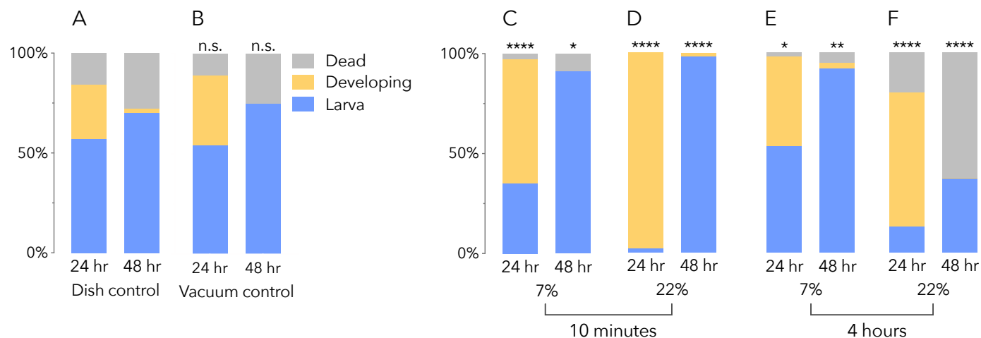
Fig. 3 Survival in the channel. (A) Percentage of wildtype embryos that reached larval stage, were still developing, or dead, 24 and 48 hours after compression ( n=111 ). (B) Vacuum controls ( n=68 ) were loaded into the channel but never compressed. (C, E) Embryos compressed at 7% ( n=34 , 38) showed greater survival rates than controls. (D) 22% compression for 10 minutes ( n=64 ) led to developmental delays but greater overall survival; (F) 22% compression for 4 hours ( n=100 ) led to death. Statistics compare observed distribution to expected from dish control (Table S1).
