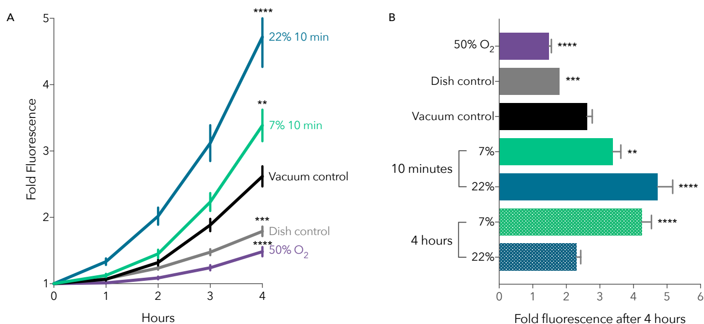
Fig. 6 Mechanical induction of twist expression. (A) twist :eGFP fluorescence was measured every hour over 4 hours after compression. Embryos show a significant increase in mean fluorescence when compressed for 10 minutes by 7% (0 PSI, p < 0.01 ) and 22% (5 PSI, p < 0.0001 ; Ordinary one-way ANOVA to vacuum control, SEM bars). Vacuum controls were introduced into the channel with the walls held open; dish controls remained outside the channel. Hypoxia (50% O 2 ) decreased twist :eGFP expression ( p < 0.0001 ). (B) Summary of twist :eGFP fluorescence after 4 hours. Embryos were exposed to three compression levels for either 10 minutes or 4 hours (SEM bars, ordinary one-way ANOVA to vacuum control).
