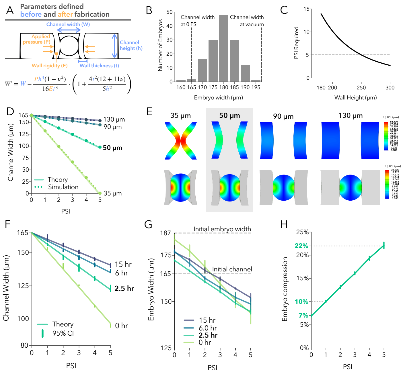
Fig. 2 Defining five parameters for a mesofluidic device: (A) Overview: The effective width of a channel under pressure ( W' ) is described by an equation with five parameters (Eq. 6). Three were defined before fabrication (blue) and two were determined afterwards (orange). The goal was to maximize compression while limiting pressure to 5 PSI for reliable function. (B) Initial channel width was determined by measuring the width distribution of stage-5 Oregon R embryos ( n=140 ). A channel width of 165 \mu\text{m} immobilizes > 99% of embryos at rest (0 PSI) while expanding under vacuum to accommodate the widest embryo. (C) Channel height: Theoretical prediction of PSI required to sufficiently deflect a wall of varying height. Height was maximized at 250 \mu\text{m} to enable compression at 5 PSI. Wall height has the greatest influence over deflection, as indicated by the polynomial degree of the governing equation. (D) Wall thickness: Deflection under pressure was calculated theoretically (solid line) and by numerical simulation (dotted line). Simulation shows < 5% difference from analytical equation 6 (Table S2). (E) Simulated deflection of sidewalls at 5 PSI in a range of thickness with and without embryos (side view cross-section). 50 \mu\text{m} walls (shaded) were selected for the greatest range of compression with the least wrapping around the embryo. (F) Wall rigidity: Longer post-cure baking results in more rigid walls (higher Young's Modulus) that deflect less under pressure. Continuous theoretical results with the discrete experimental measurements from 1 PSI increments (95% CI bars). (G) Embryo width between walls with a range of rigidity (95% CI bars). 2.5 hours post-cure bake showed the greatest range of compression with minimal wrapping. (H) Uniaxial compressive strain (normalized change in embryo width) in the final channel after design optimization (95% CI bars).
